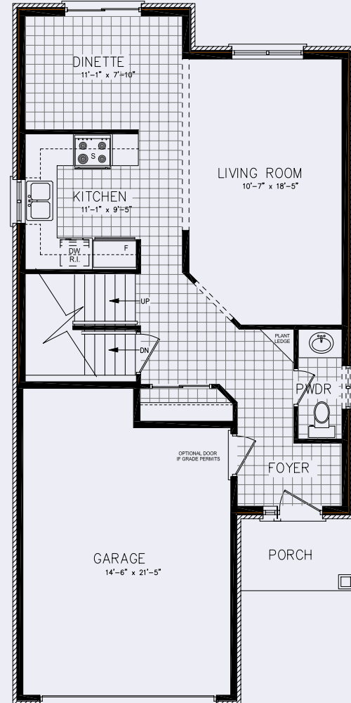
MAIN FLOOR
