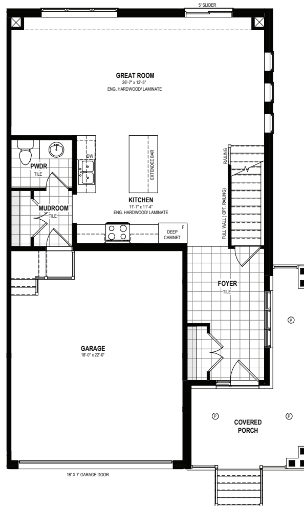
MAIN FLOOR
