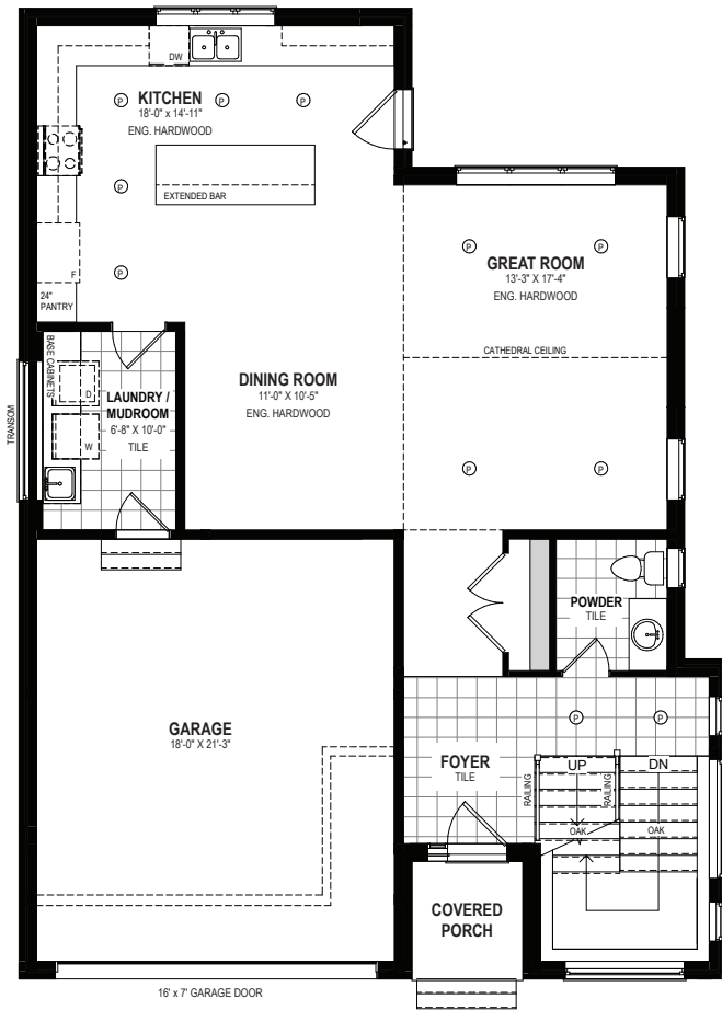
MAIN FLOOR
