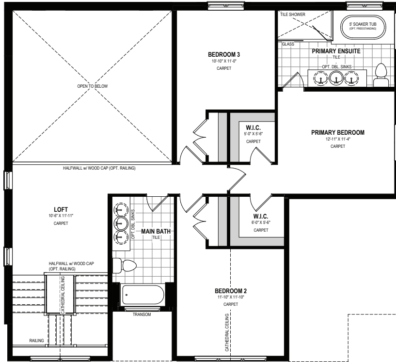
SECOND FLOOR
