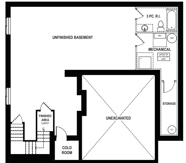
BASEMENT
