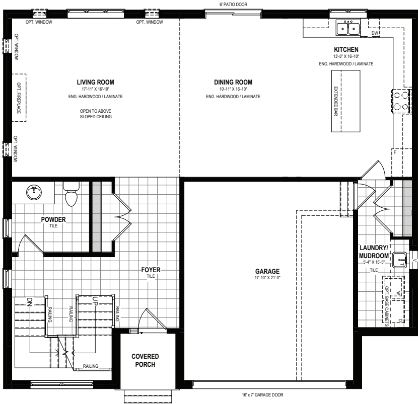
MAIN FLOOR
