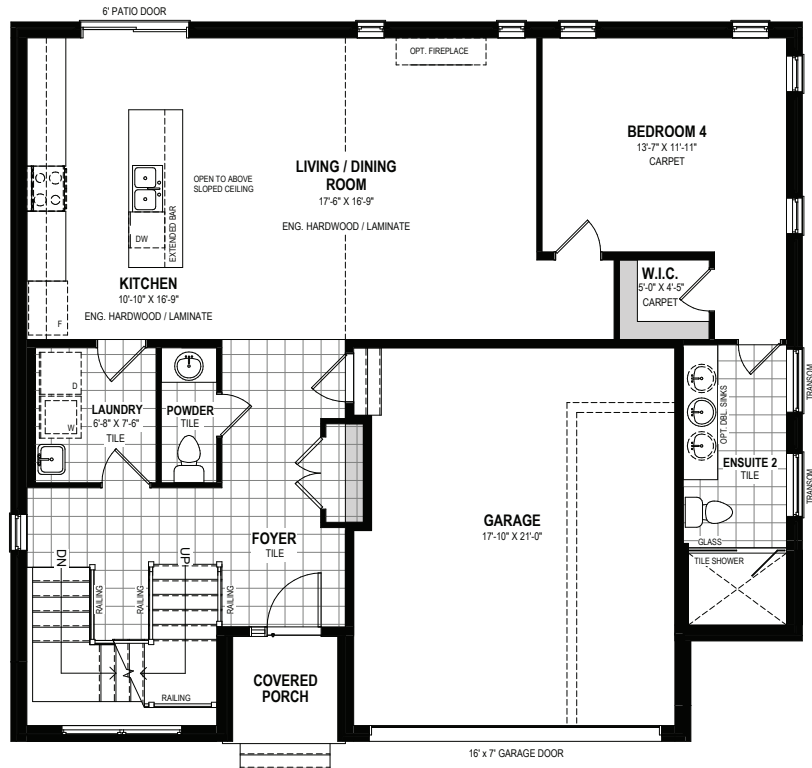
MAIN FLOOR
