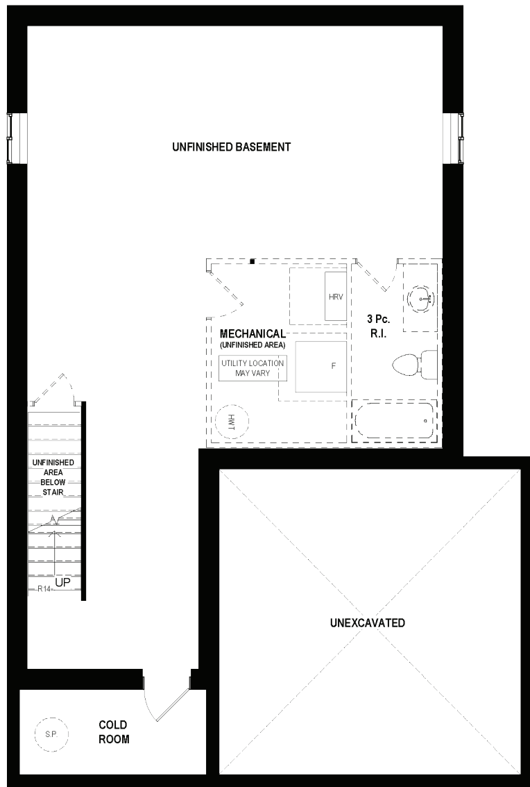
BASEMENT FLOOR
