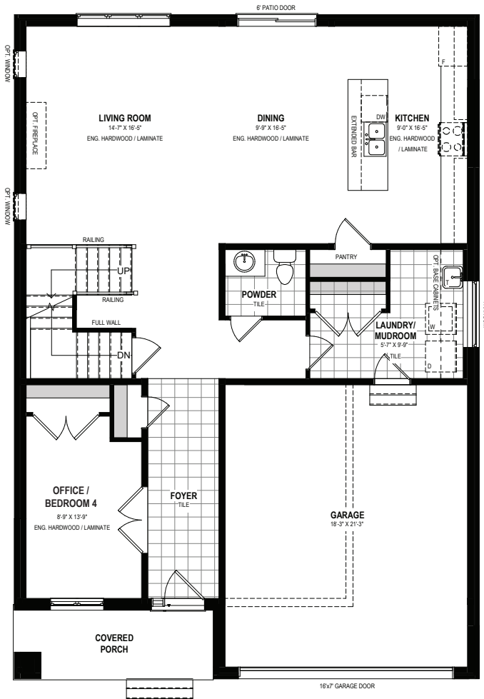
MAIN FLOOR
