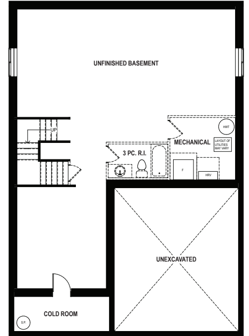
BASEMENT
