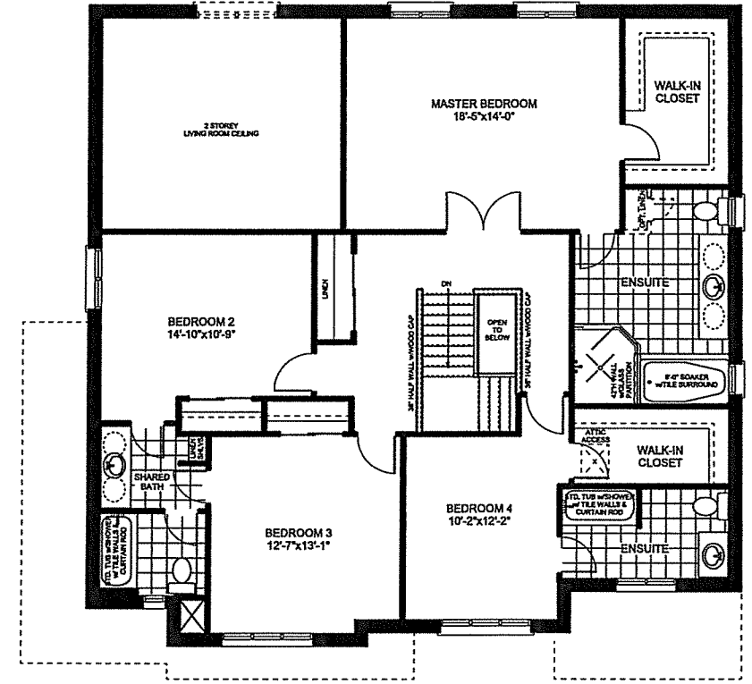
UPPER FLOOR PLAN FINISHED FLOOR AREA: 1568 SQ.FT.
