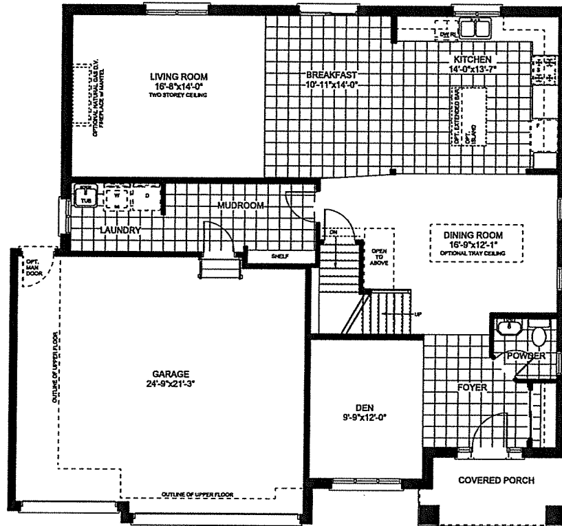
MAIN FLOOR PLAN FINISHED FLOOR AREA: 1386 SQ.FT.
