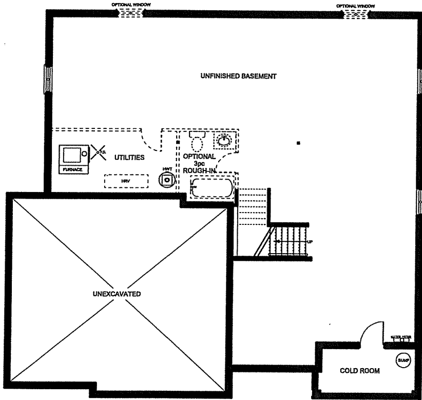
BASEMENT PLAN
